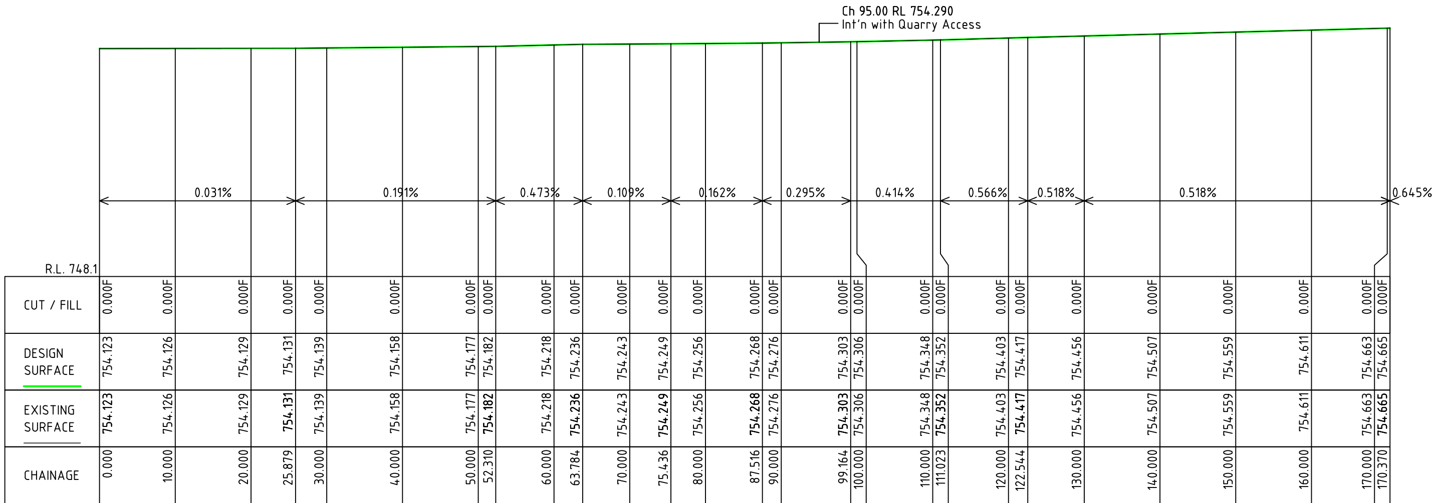
LONGITUDINAL SECTION Ch 0.000 to Ch 170.370 SCALES: HORIZONTAL 1:500 VERTICAL 1:100
